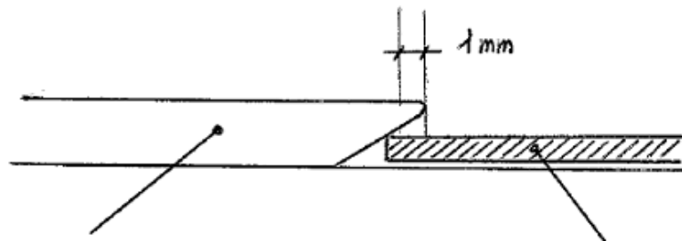
Cover plate with reverse taper
